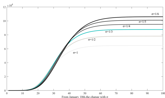
Figure 10: The changes of different \sigma in the cumulative of confirmed cases in mainland China during the COVID-19 transmission process.
